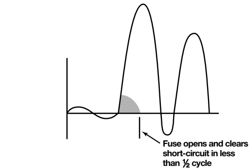
A current-limiting fuse has such a high speed of response that it cuts off a short-circuit long before it can build up to its full peak value.
